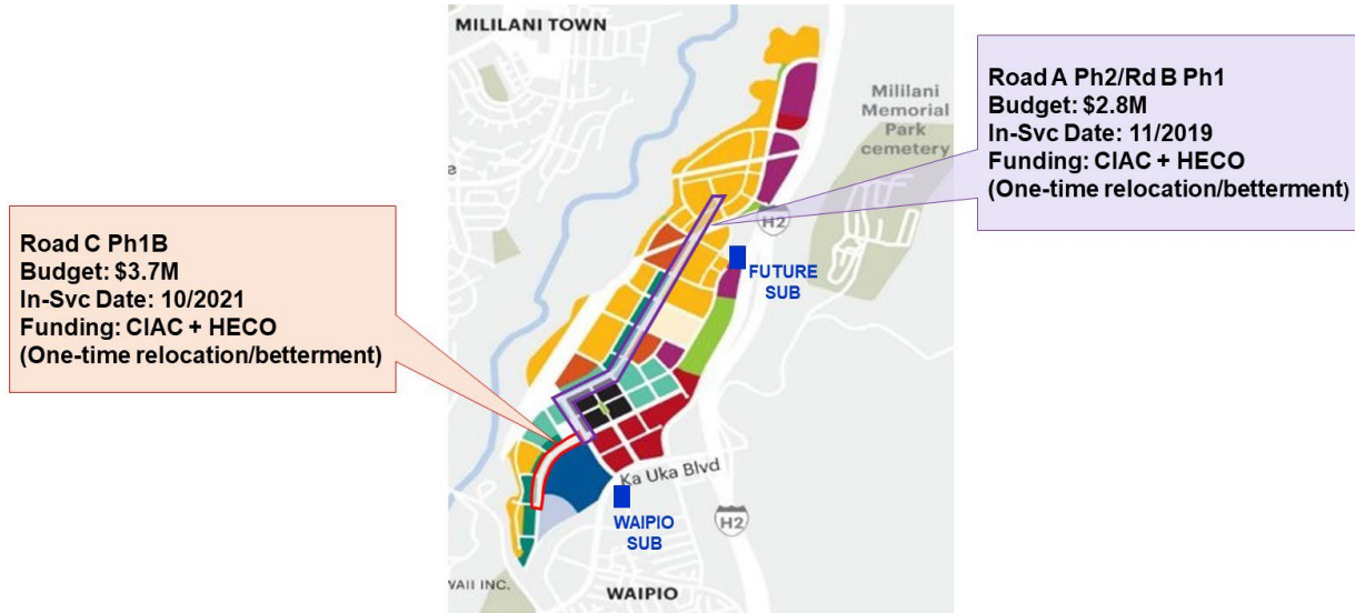
Figure F-7: Waiiau-Mililani 46 kV OH to UG Conversion
