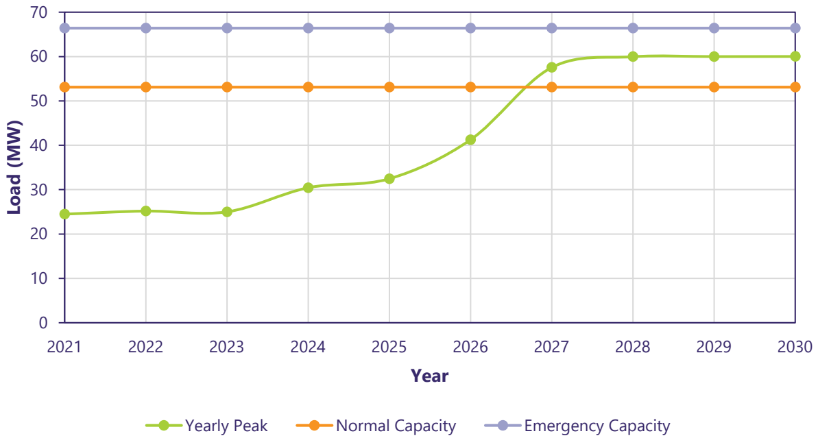
Figure F-12: Kewalo T3 2027 Peak Day Overload
