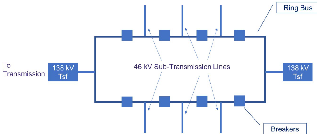
Figure F-8: Waiiau 46 kV GIS Bus
