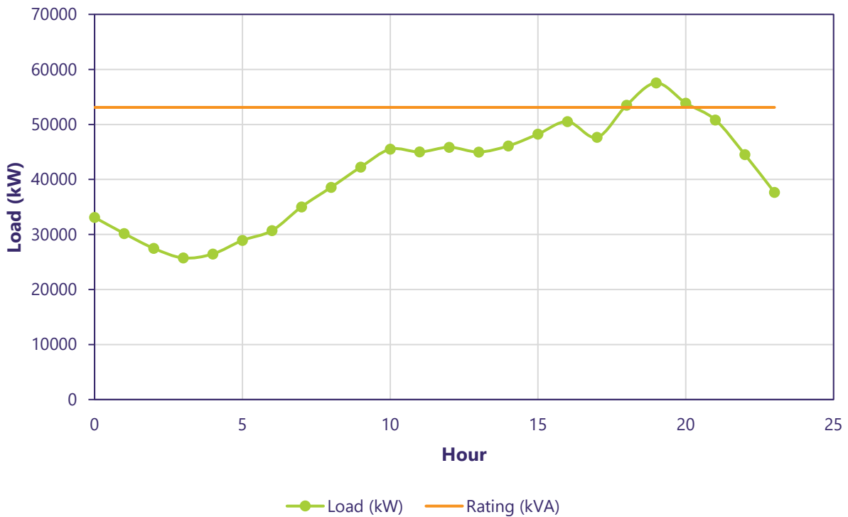
Figure F-12: Kewalo T3 2027 Peak Day Overload
