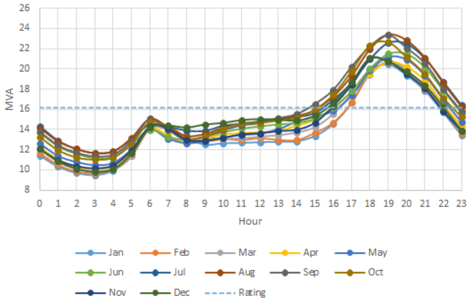
Figure F-16: Kalo #1 Transformer Loading – Monthly Peak Day in 2023
